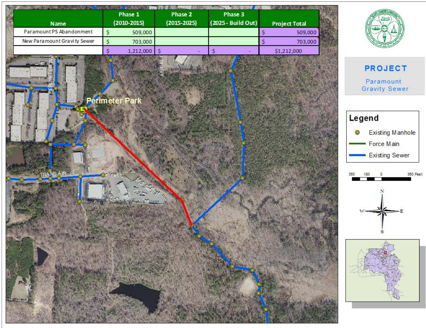
Figure 7-39: New Paramount Gravity Sewer
