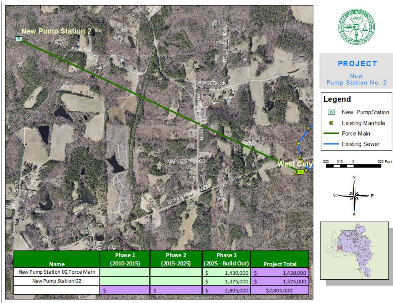
Figure 7-34: New Pump Station No. 2 and Force Main
