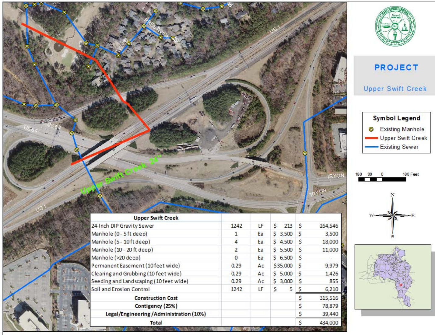
Figure 7-32: Upper Swift Creek Interceptor
