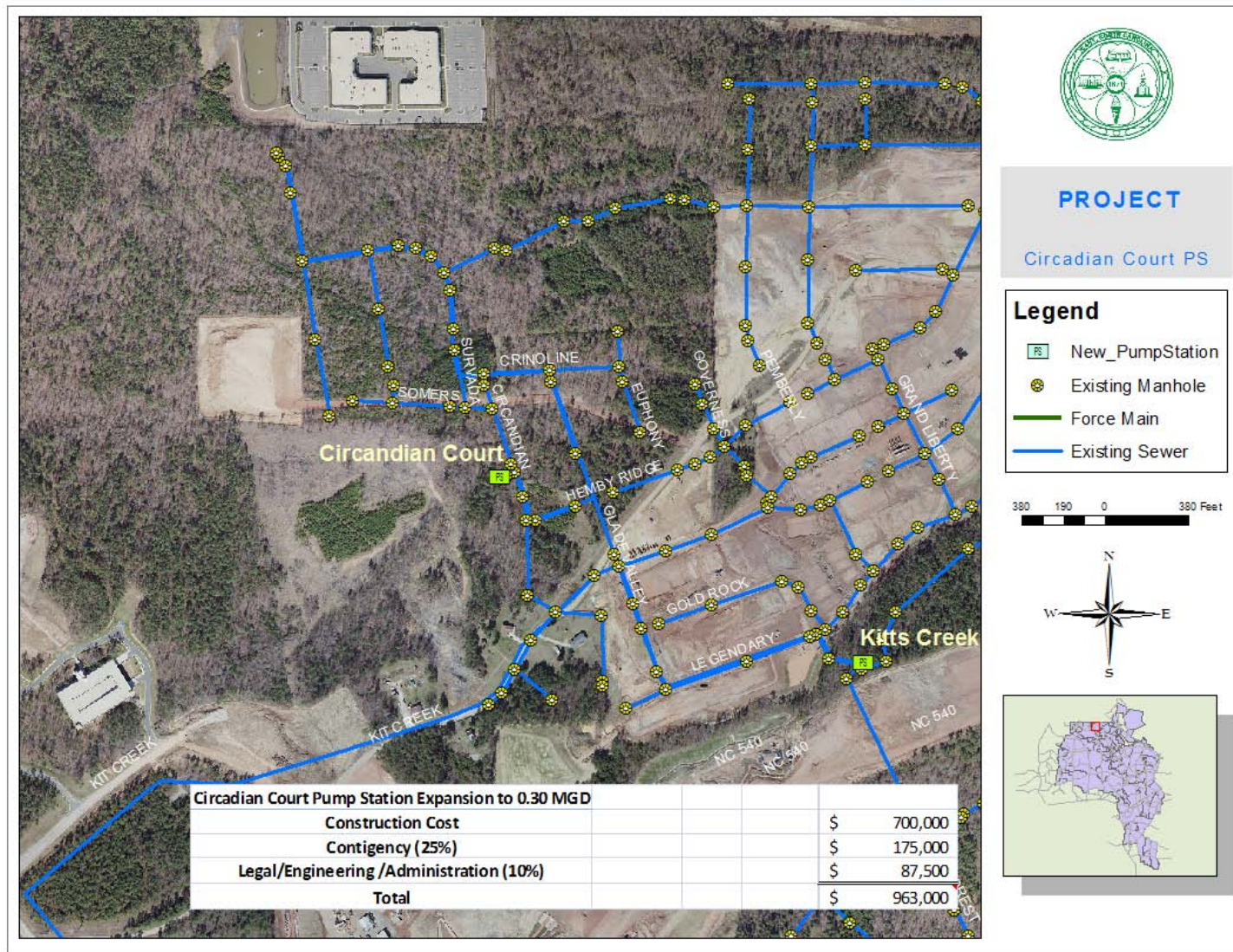
Figure 7-29: Circadian Court Pump Station Upgrade
