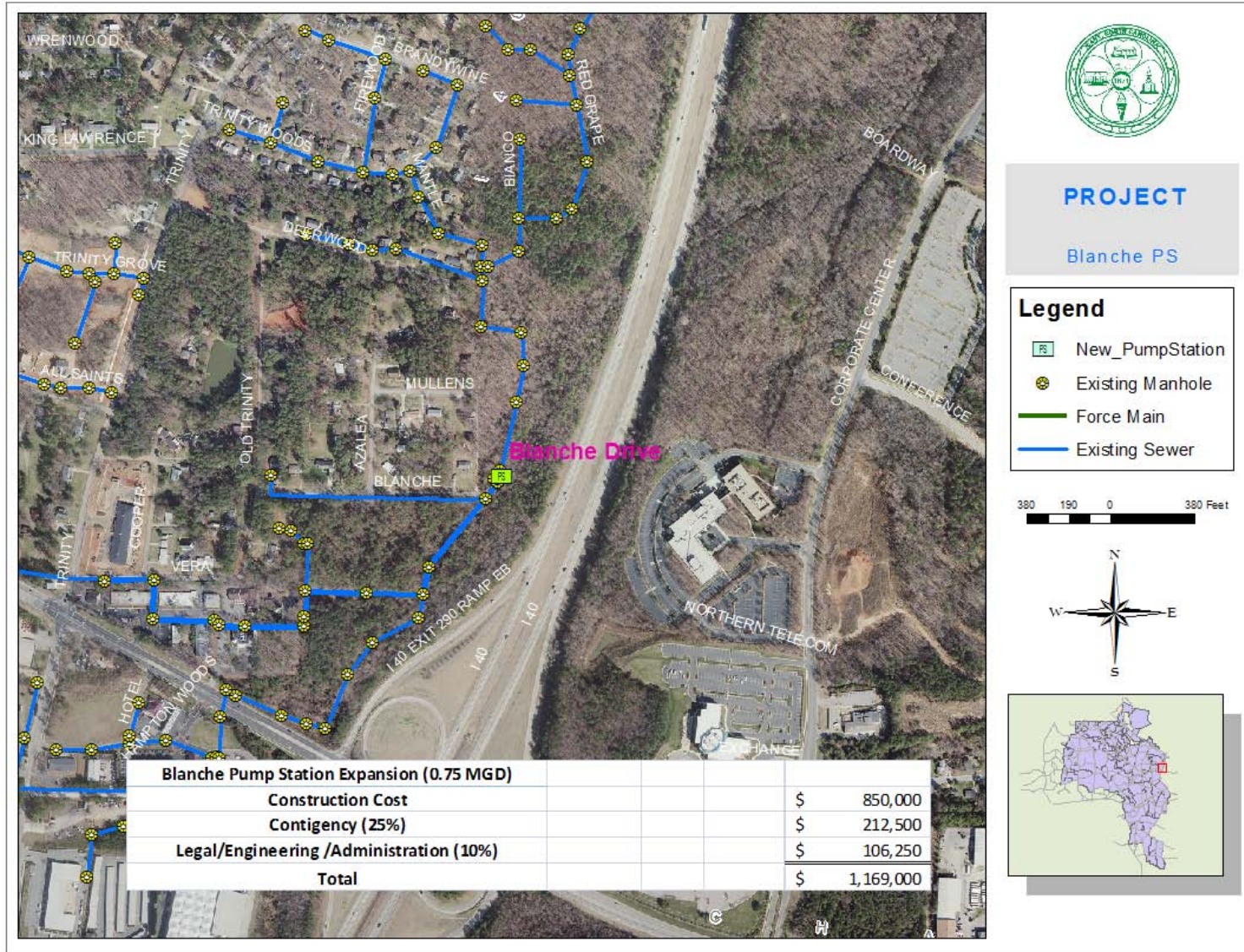
Figure 7-22: Blanche Pump Station Upgrade
