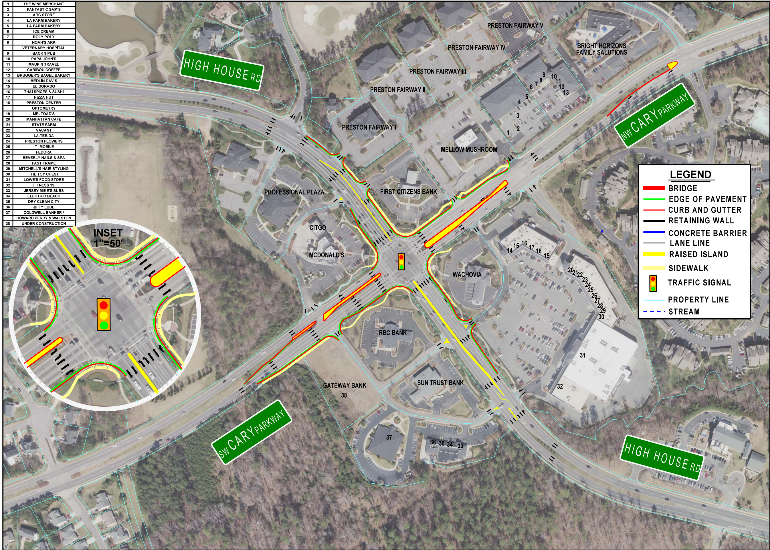
Cary Parkway/High House Road Intersection Improvements Figure 4-3: Alternative #1: Turn Lane Improvements Conceptual Design
