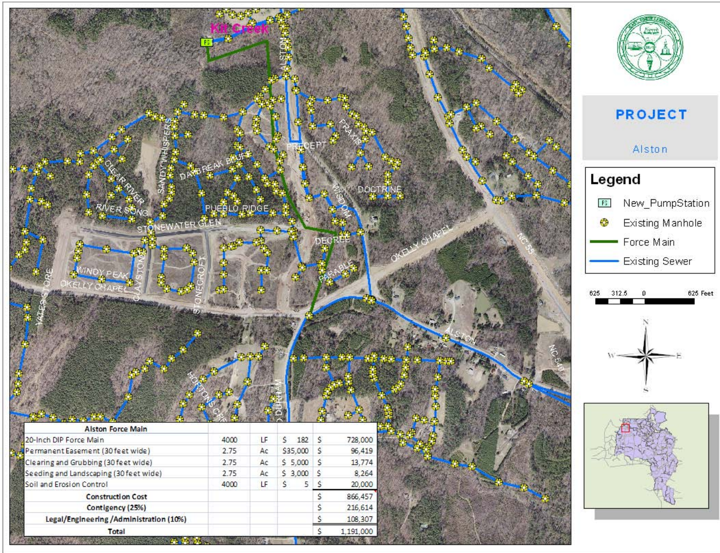
Figure 7-16: Details of Alston Force Main
