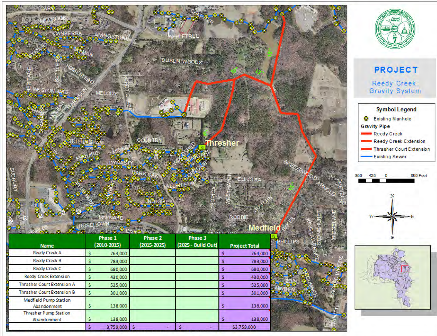
Figure 7-14: Reedy Creek Regional Pump Station and Related Gravity Sewers
