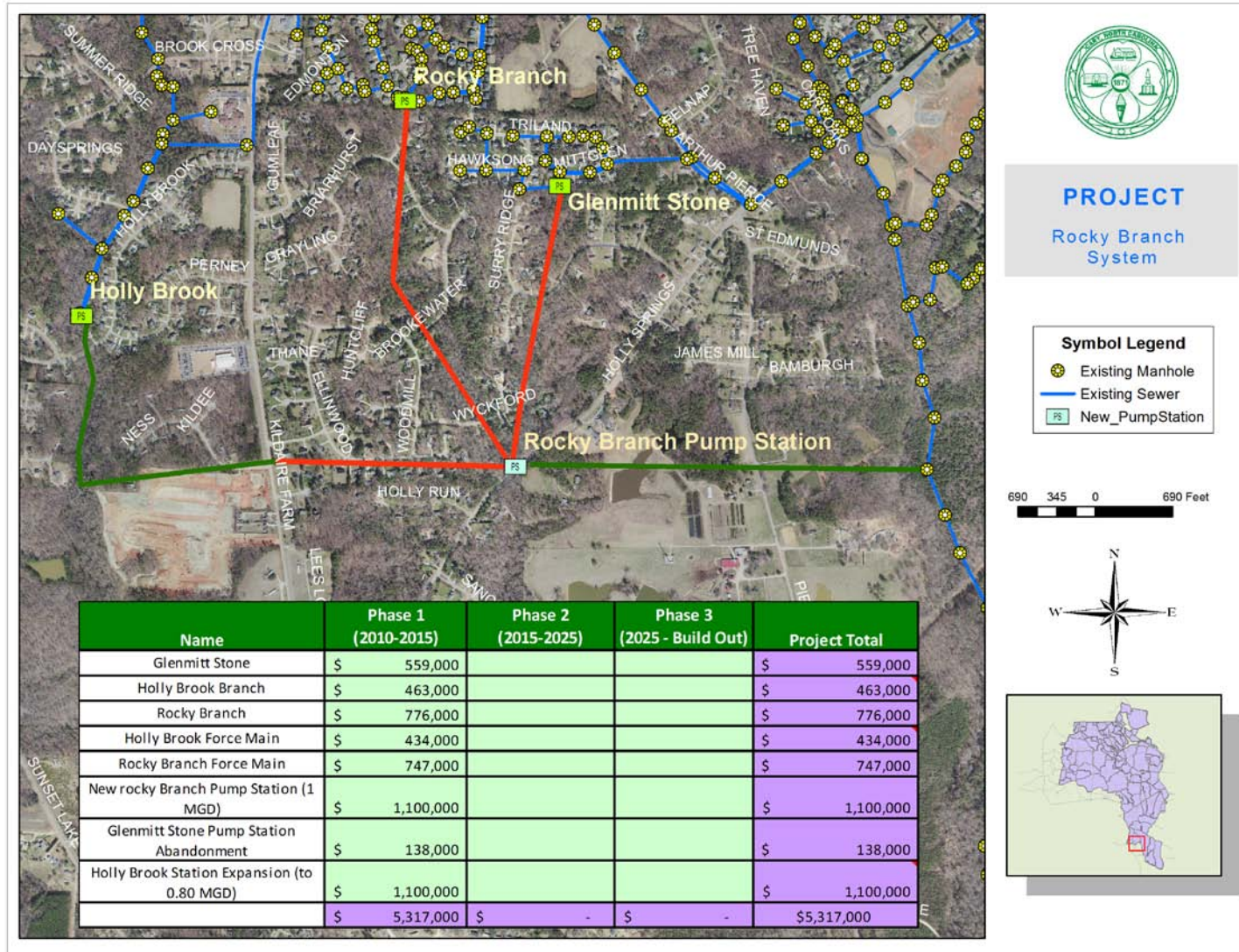
Figure 7-12: Rocky Branch Pump Station and Related Sewers
