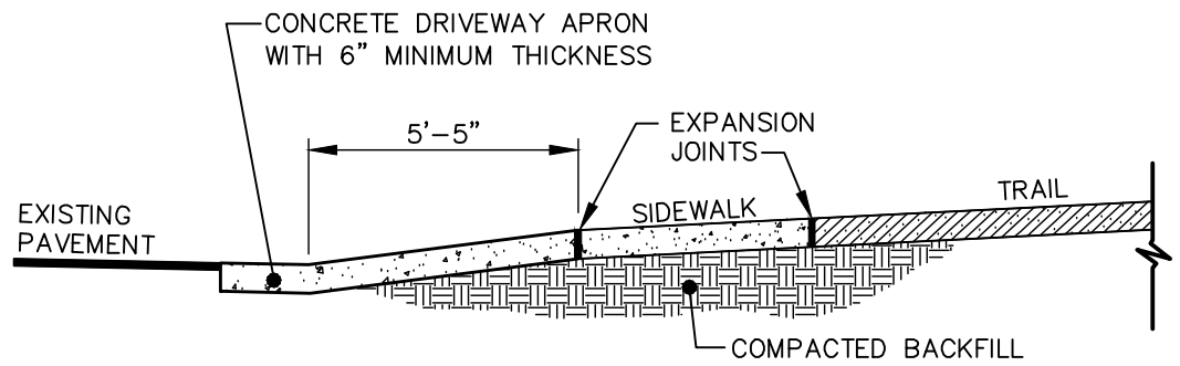
TYPICAL SECTION
