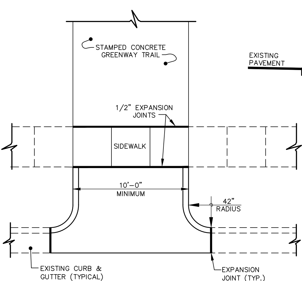
PLAN VIEW
