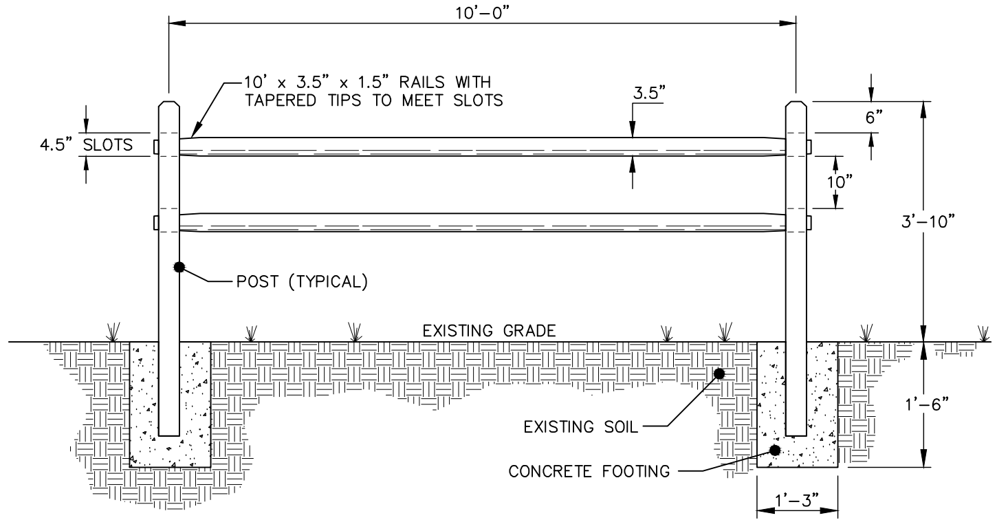
FRONT VIEW
