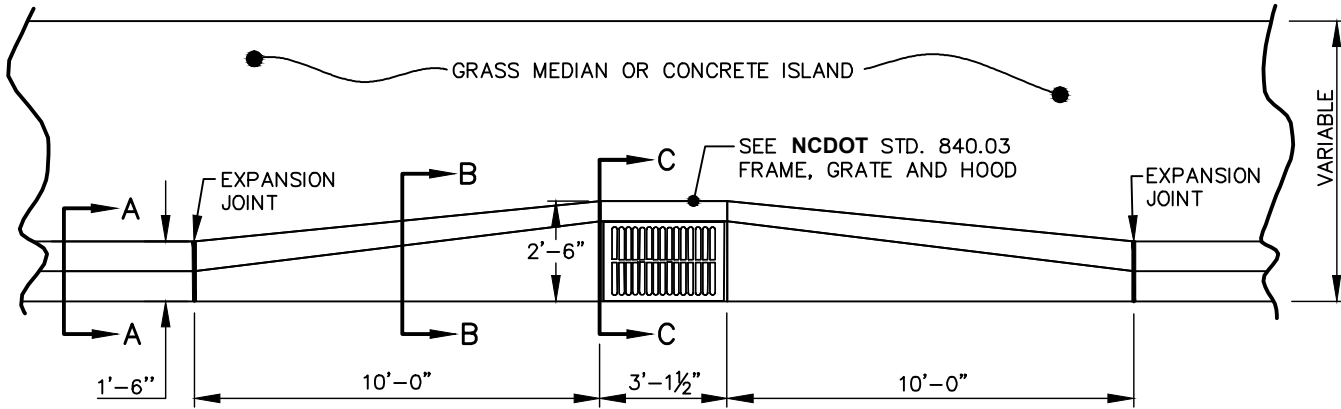
PLAN VIEW
