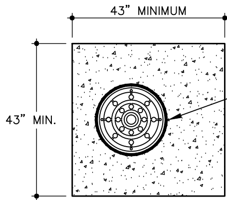
CONCRETE SLAB
