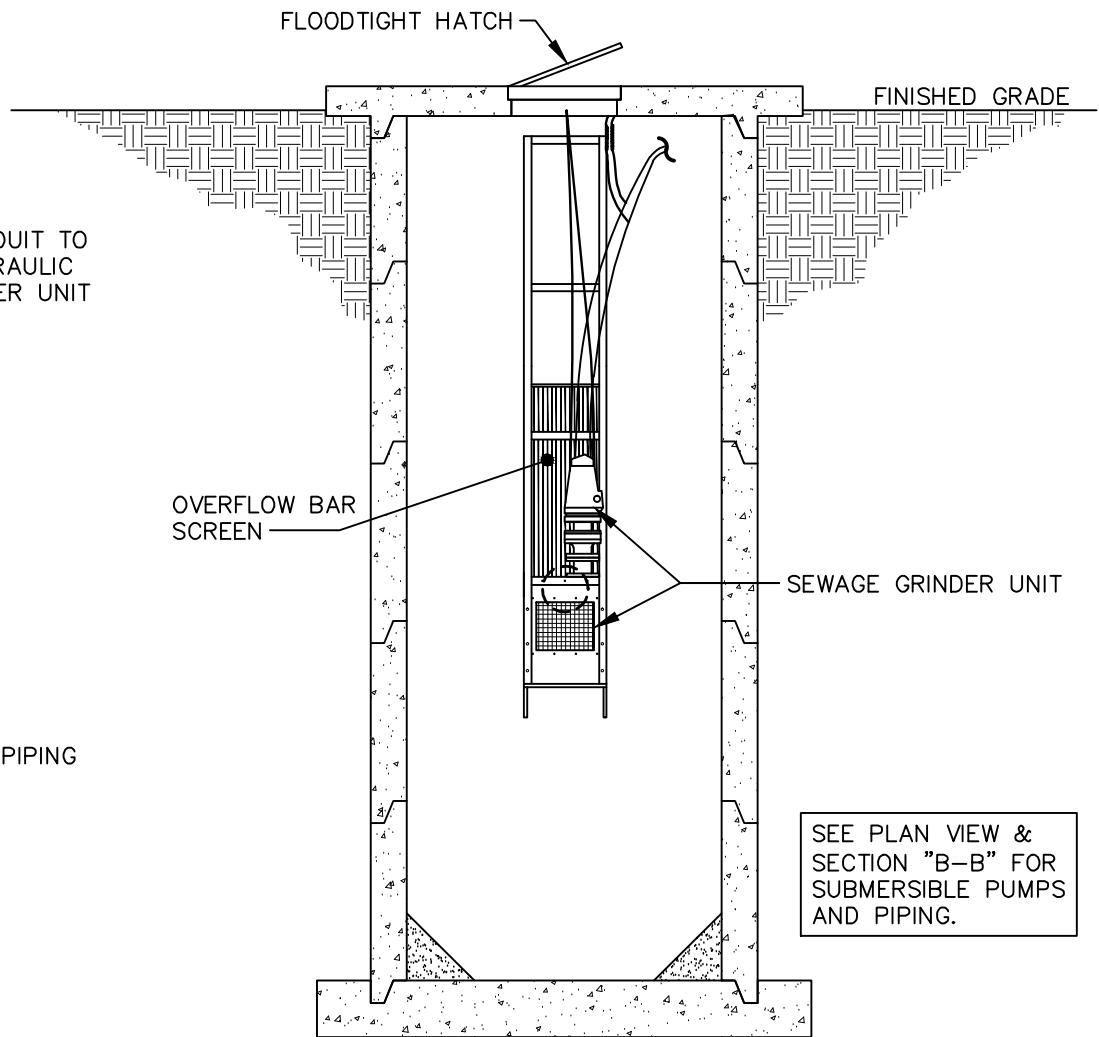
SECTION "A-A"
