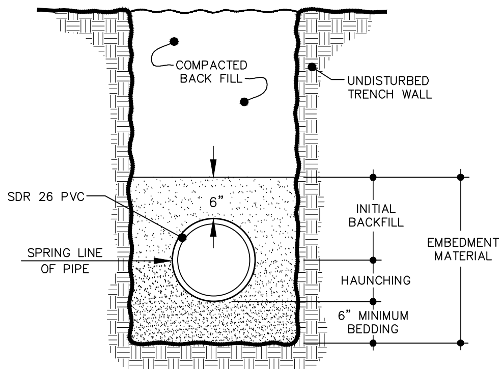
SPECIAL BEDDING FOR 14'-30' DEPTHS
