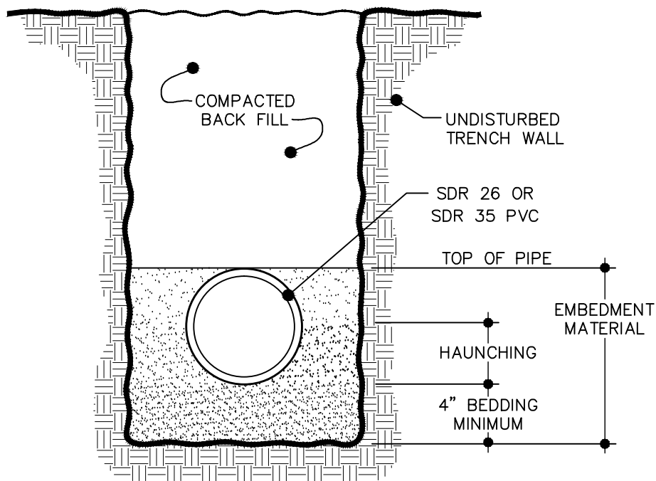
STANDARD BEDDING FOR 3' TO 14' DEPTHS
