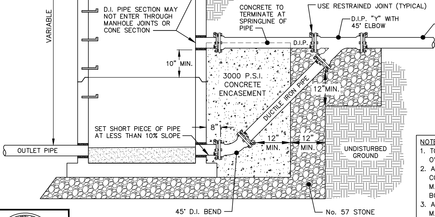
SECTION VIEW
