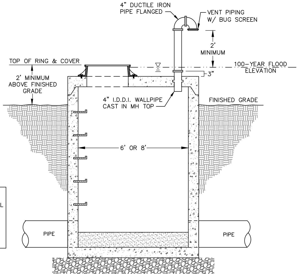
ELEVATION VIEW
