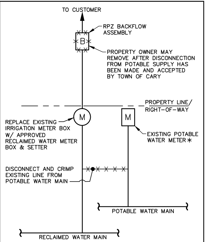
SCENARIO 3 RETROFIT OF EXISTING IRRIGATION METER ASSEMBLY FROM POTABLE TO RECLAIMED SERVICE
