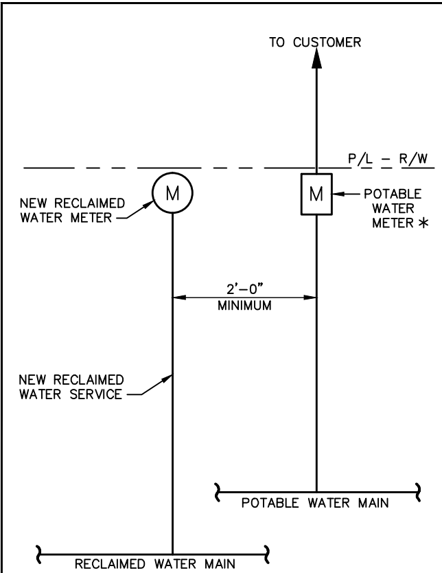
SCENARIO 1 RECLAIMED SERVICE CONNECTION (NEW INSTALLATION)
