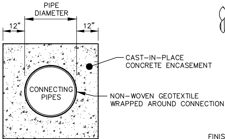
CONCRETE ENCASEMENT CROSS SECTION
