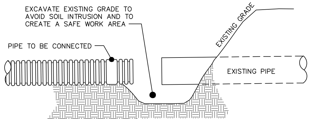
EXISTING SITE SECTION VIEW
