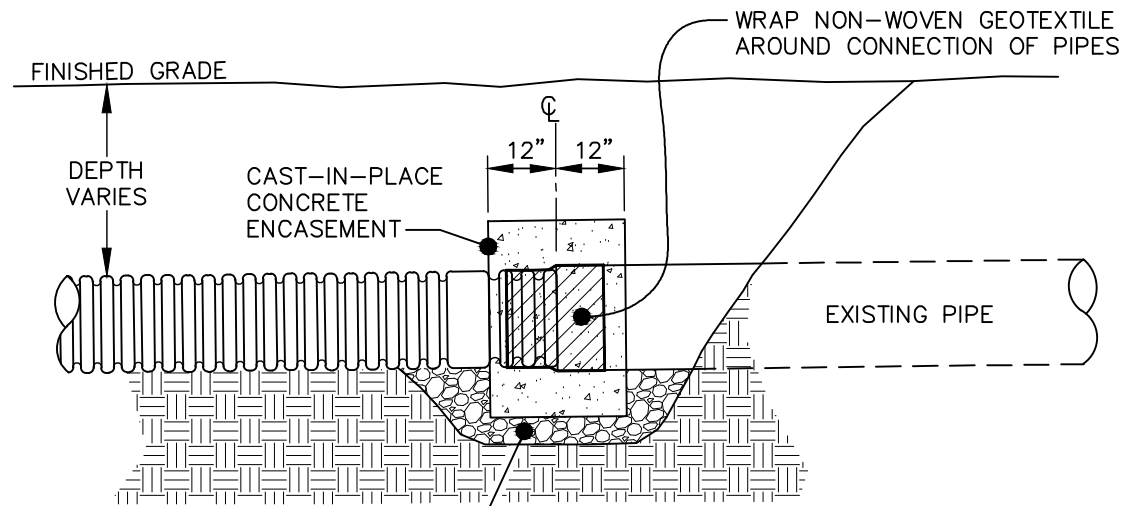
FINISHED CONNECTION SECTION VIEW
