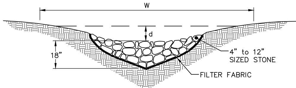
V-SHAPED WATERWAY WITH STONE CENTER DRAIN (SHAPED BY MOTOR GRADER)
