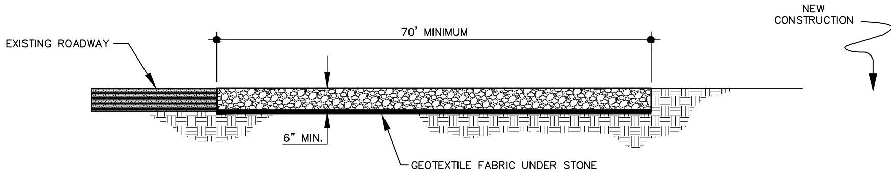
CROSS SECTION
