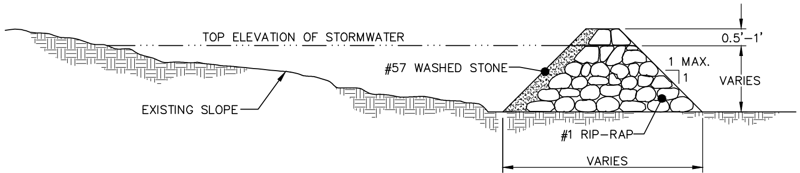
SIDE VIEW
