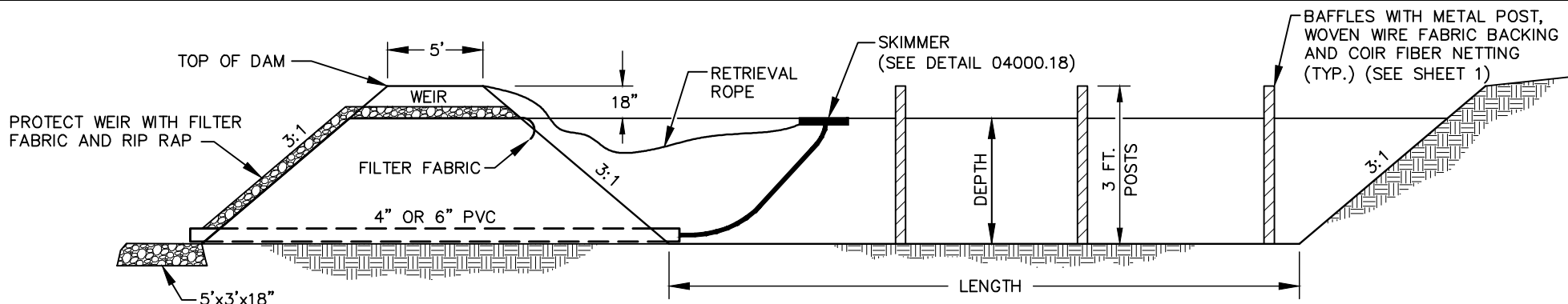
SKIMMER BASIN CROSS SECTION
