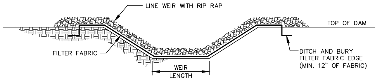
WEIR CROSS SECTION
