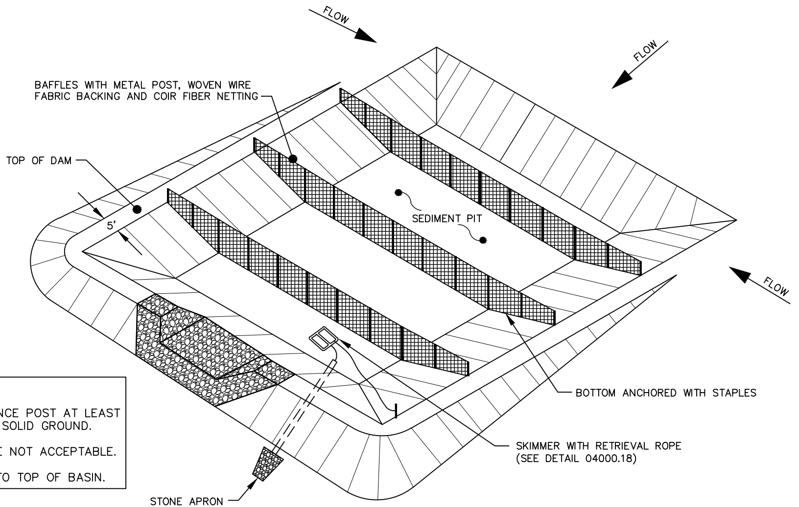
PERSPECTIVE VIEW
