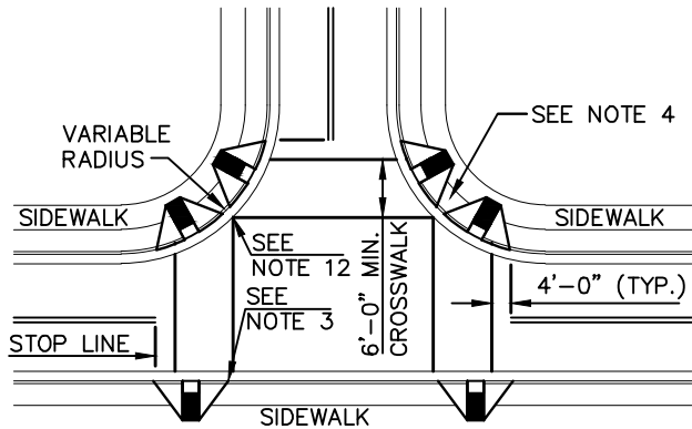
DETAILS SHOWING TYPICAL LOCATION OF WHEELCHAIR RAMPS, PEDESTRIAN CROSSWALKS AND STOP LINES FOR TEE INTERSECTIONS
