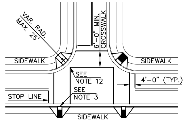
DETAILS SHOWING TYPICAL LOCATION OF WHEELCHAIR RAMPS, PEDESTRIAN CROSSWALKS AND STOP LINES FOR TEE INTERSECTIONS
