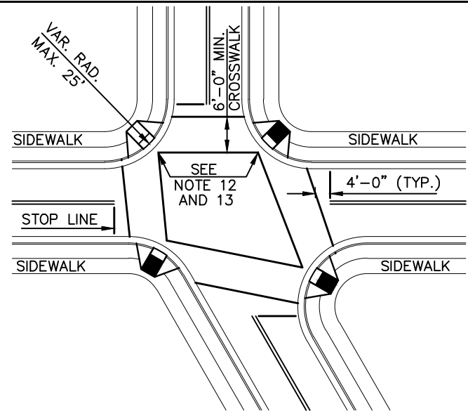
DETAILS SHOWING TYPICAL LOCATION OF WHEELCHAIR RAMPS, PEDESTRIAN CROSSWALKS AND STOP LINES
