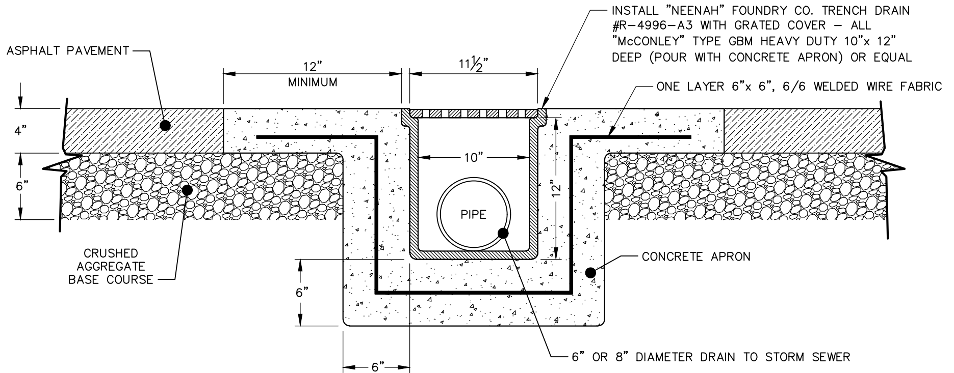
SECTION VIEW
