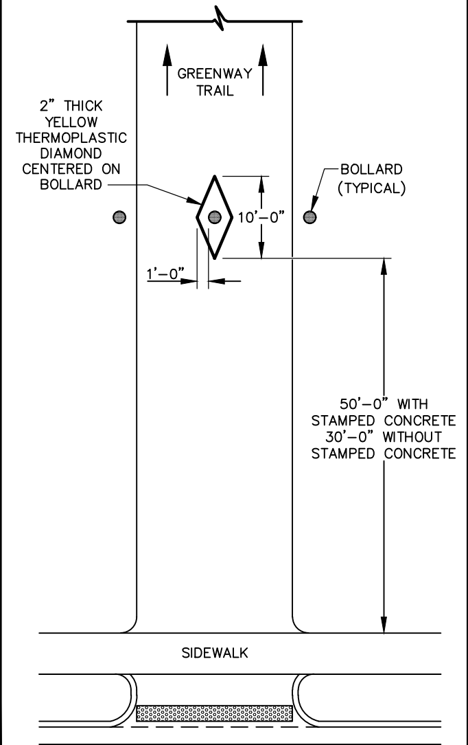
PLAN VIEW
