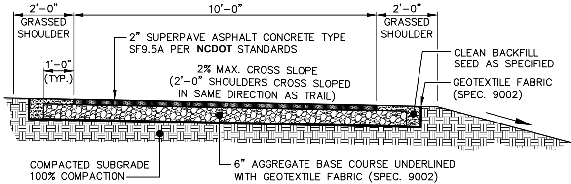
TYPICAL SECTION
