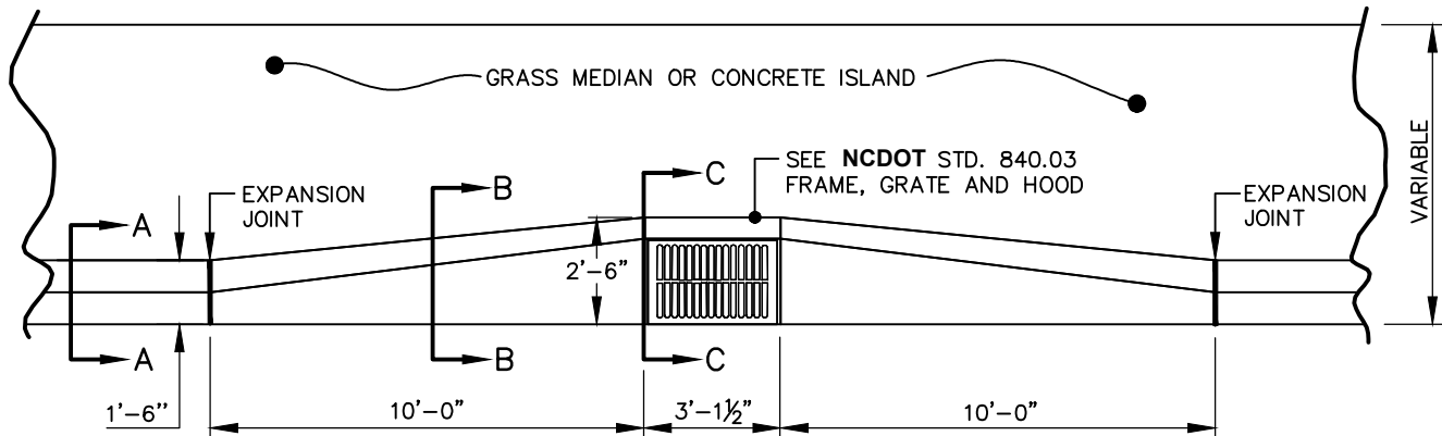
PLAN VIEW
