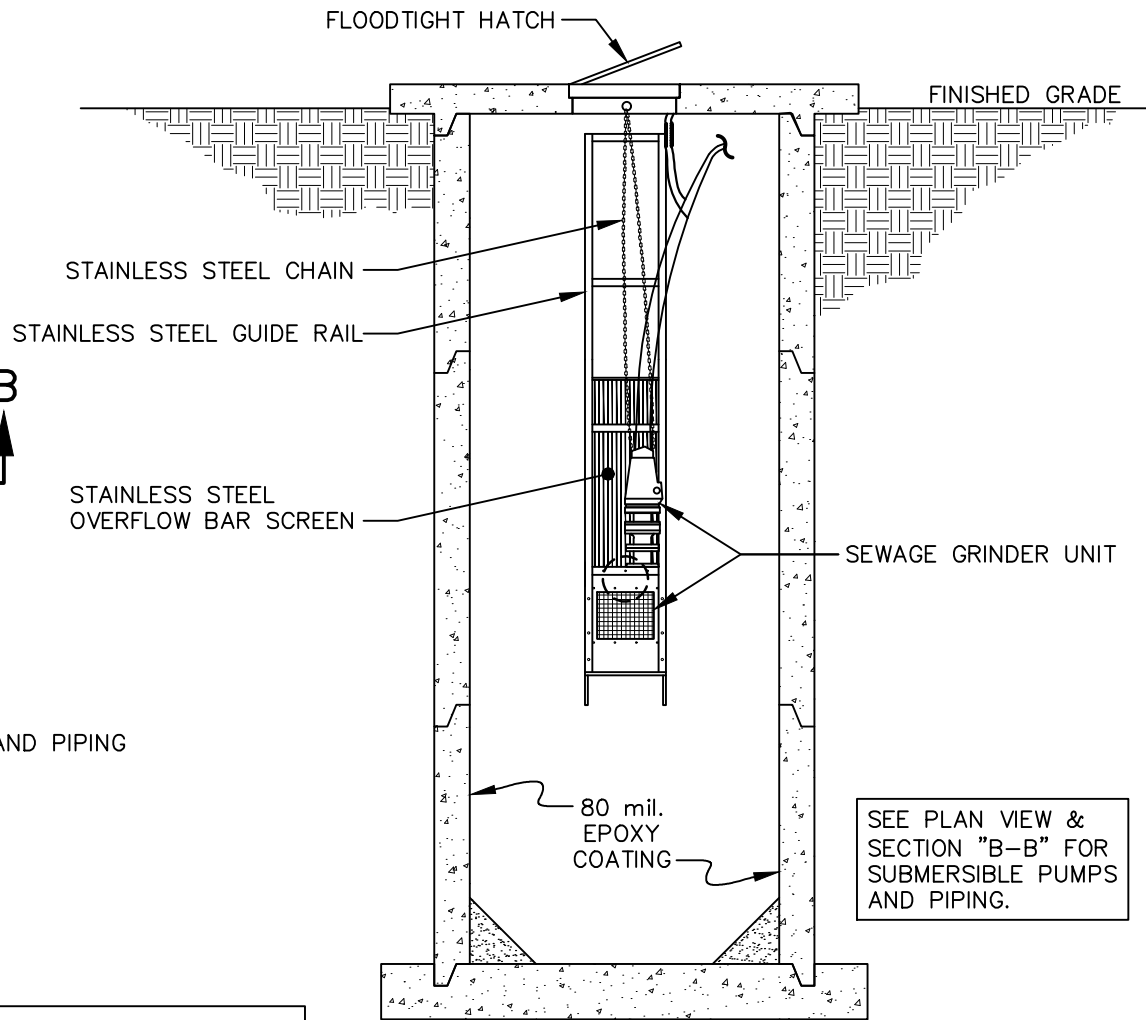
SECTION "A-A"
