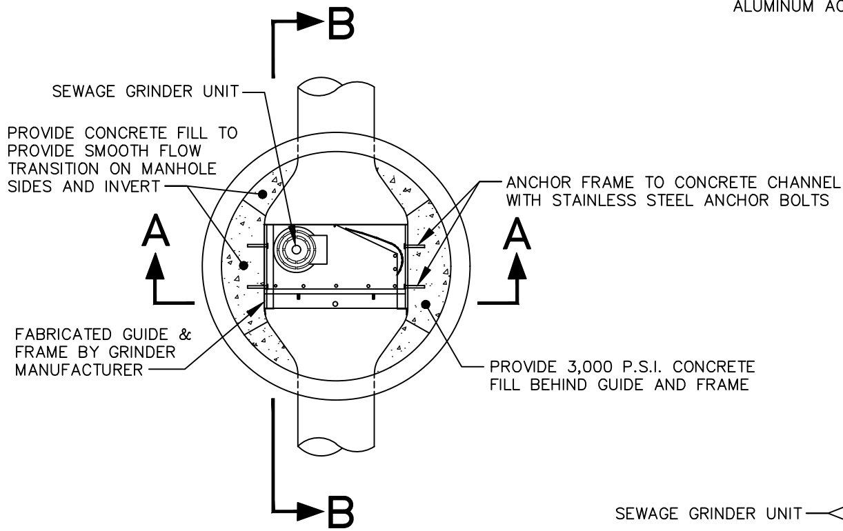
PLAN VIEW
