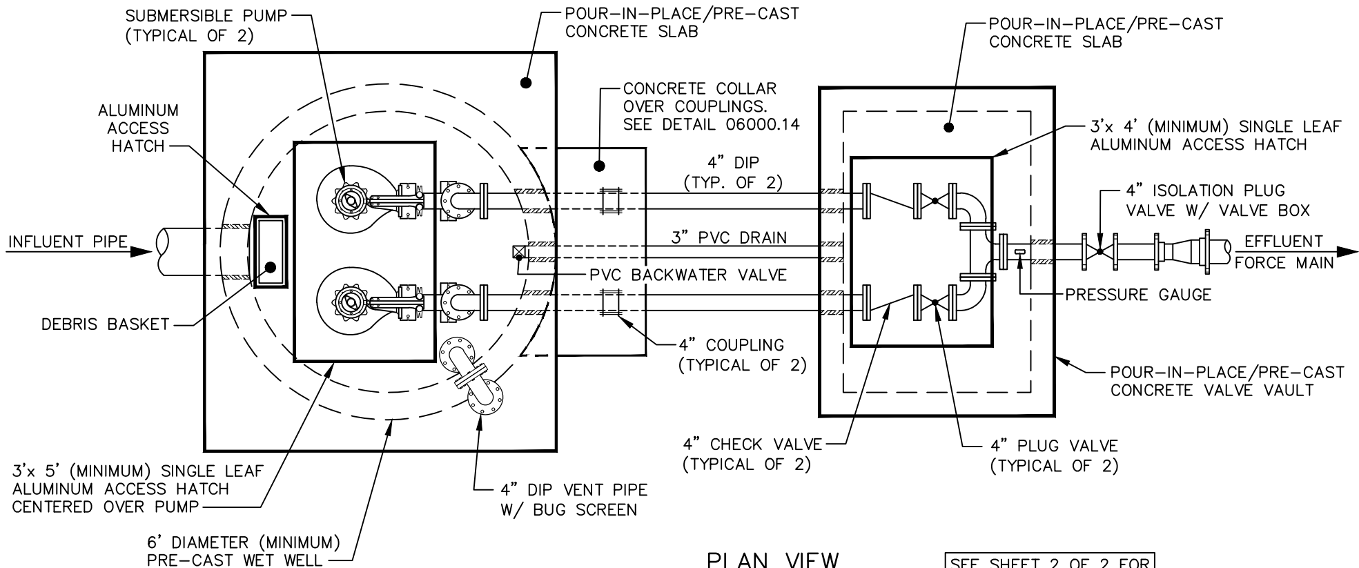
PLAN VIEW
