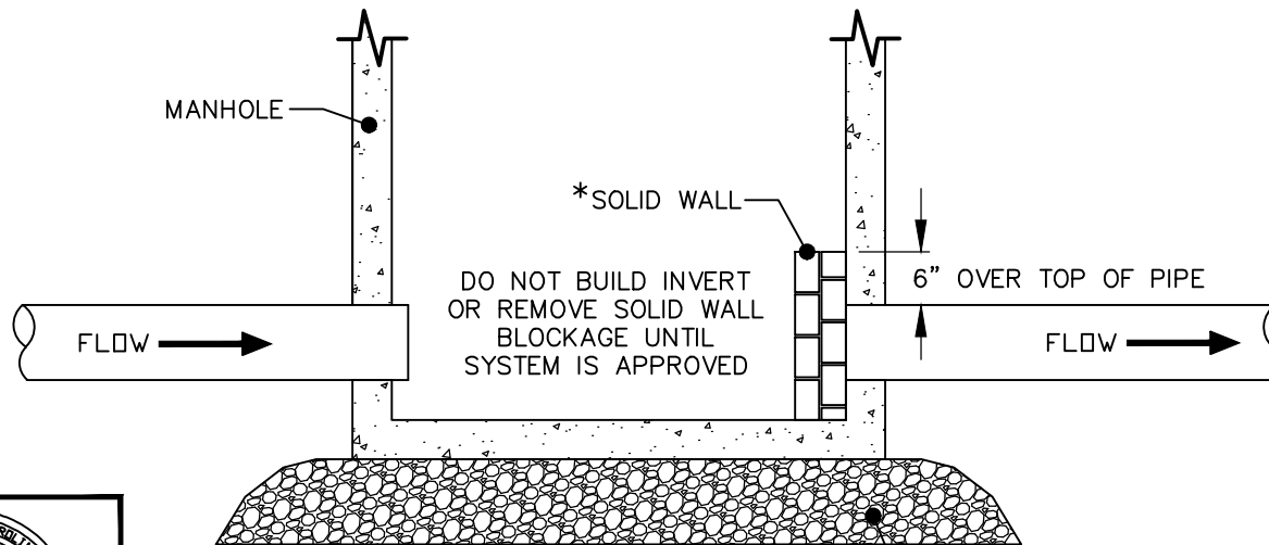
SECTION VIEW
