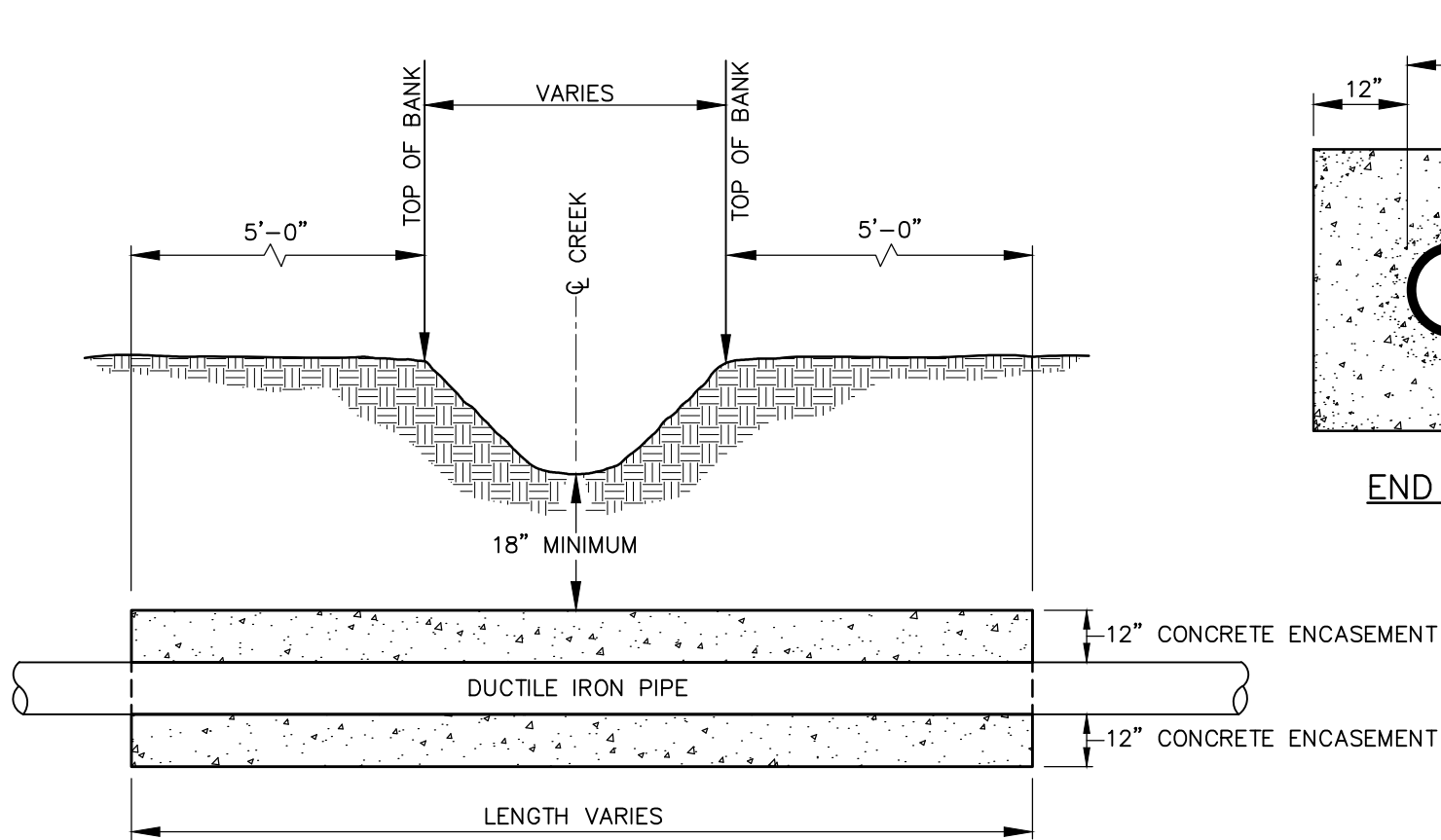
CROSS SECTION
