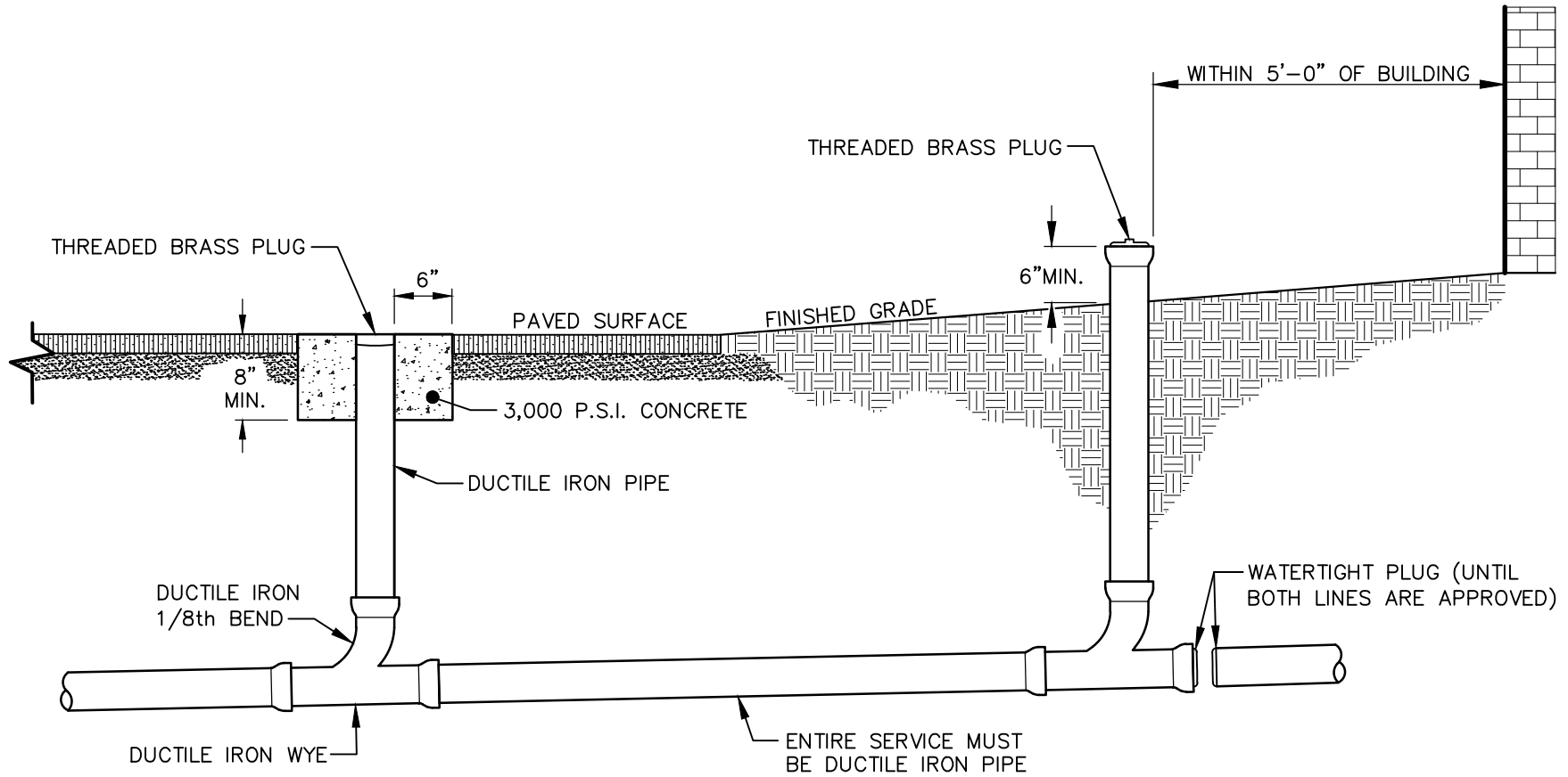
SECTION VIEW
