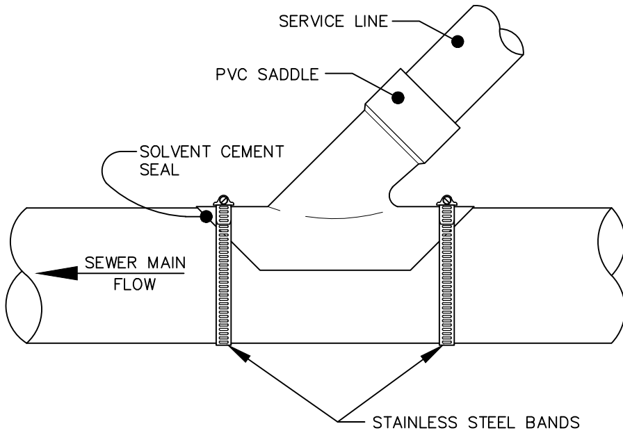
PVC MAIN
