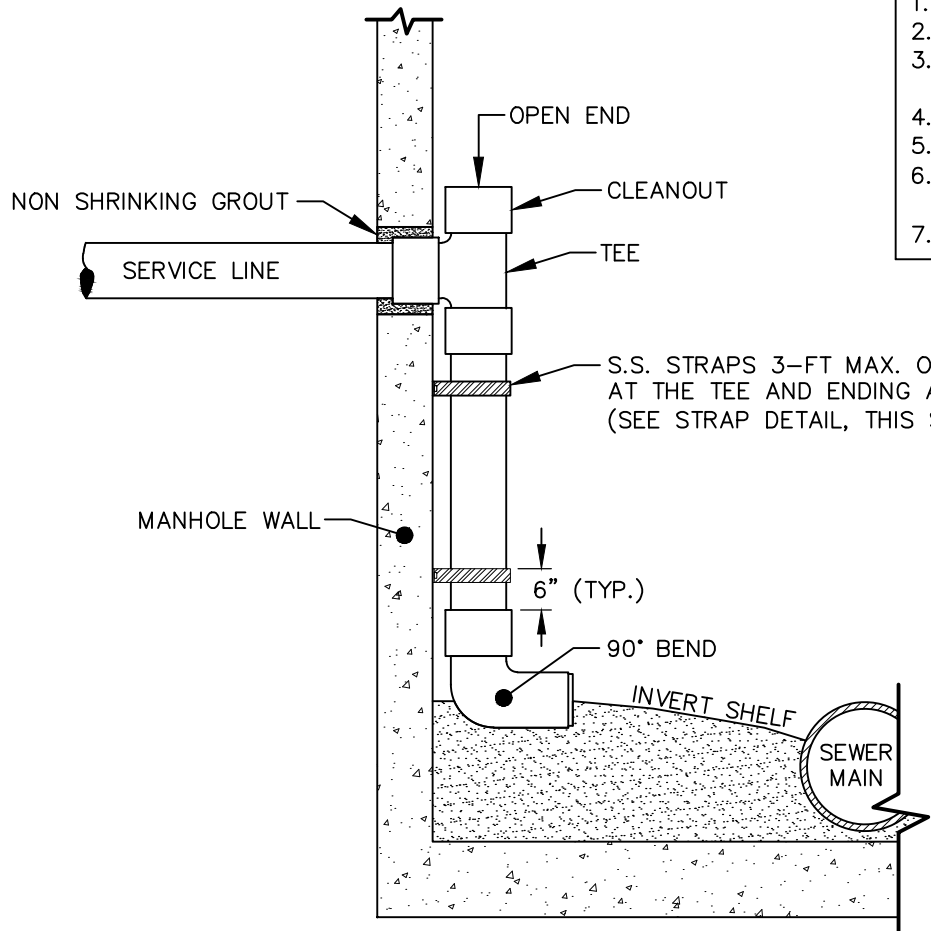
SECTION VIEW
