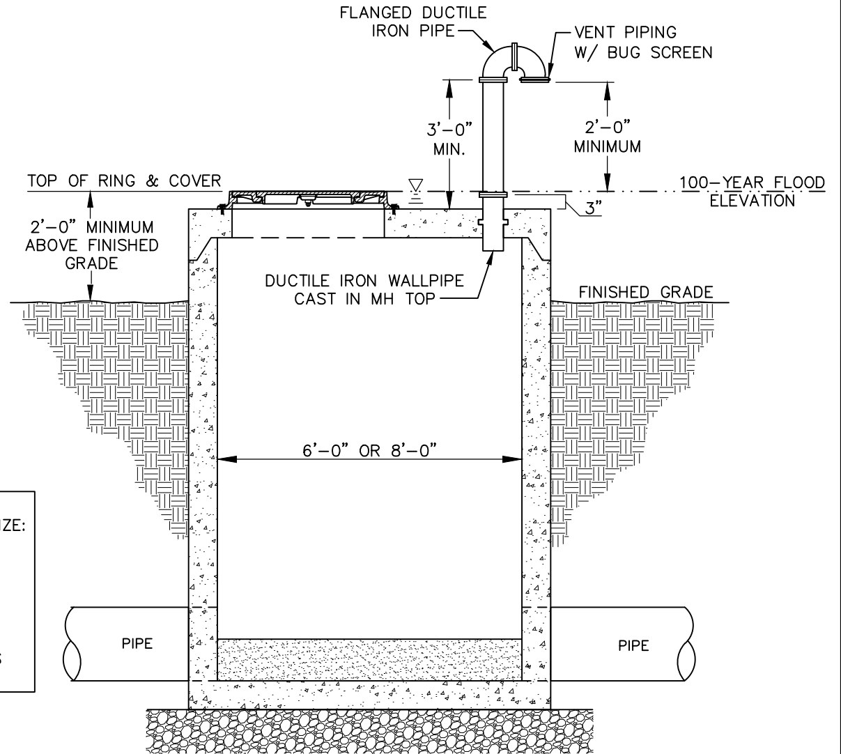
SECTION VIEW
