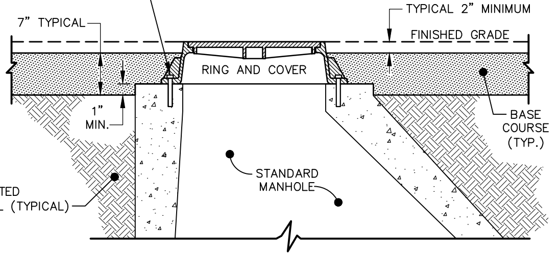
SECTION VIEW
