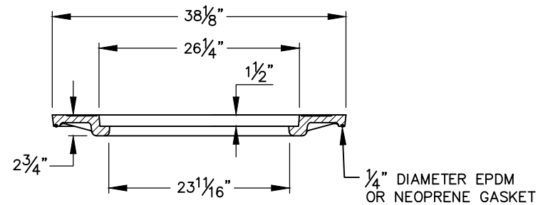
OUTER COVER SECTION
