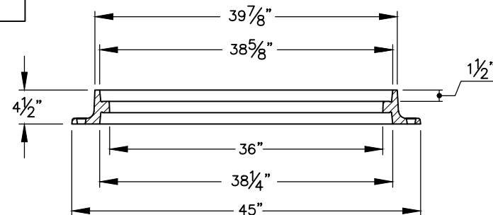
FRAME SECTION
