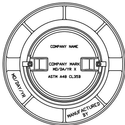
BOTTOM VIEW COVERS
