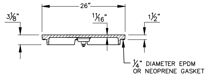
INNER COVER SECTION
