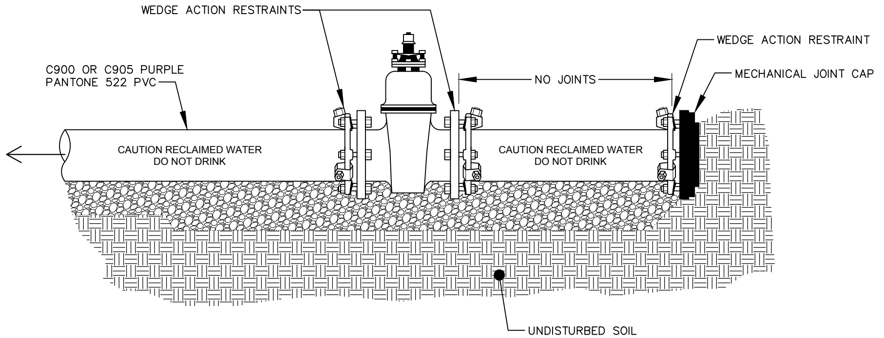
SECTION VIEW
