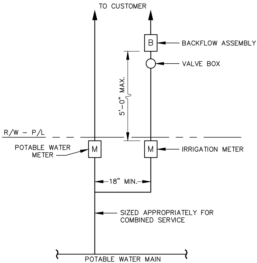
ALTERNATE 1 RETROFIT
