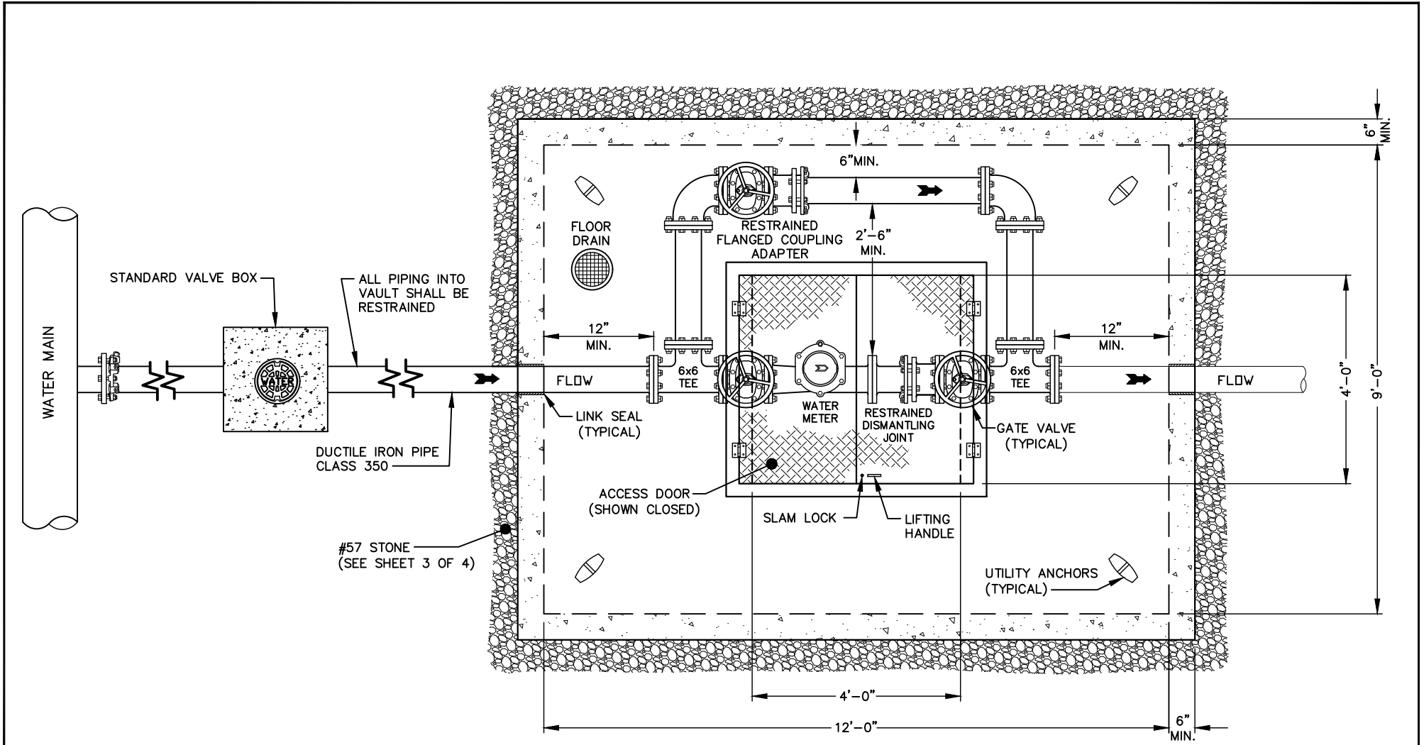
PLAN VIEW (SEE SHEET 3 OF 4 FOR SECTION VIEW)
