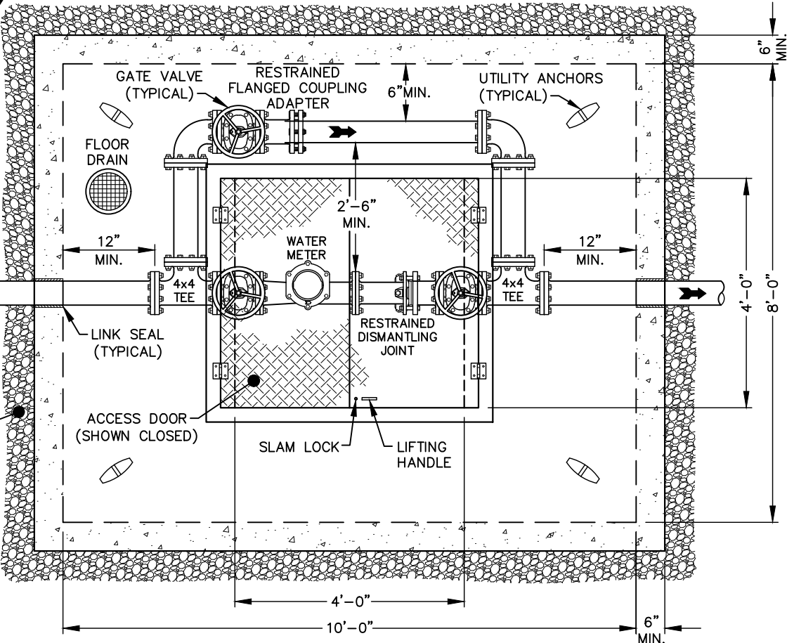
PLAN VIEW (SEE SHEET 1 OF 4 FOR SECTION VIEW)
