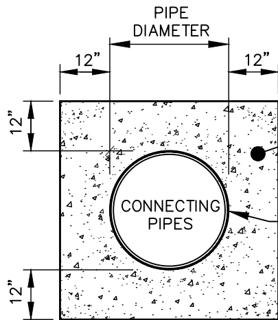
CONCRETE ENCASEMENT CROSS SECTION
