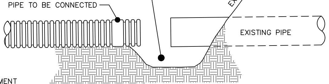
EXISTING SITE SECTION VIEW
