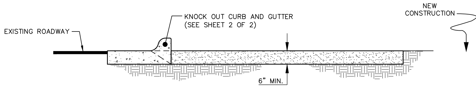
CROSS SECTION
