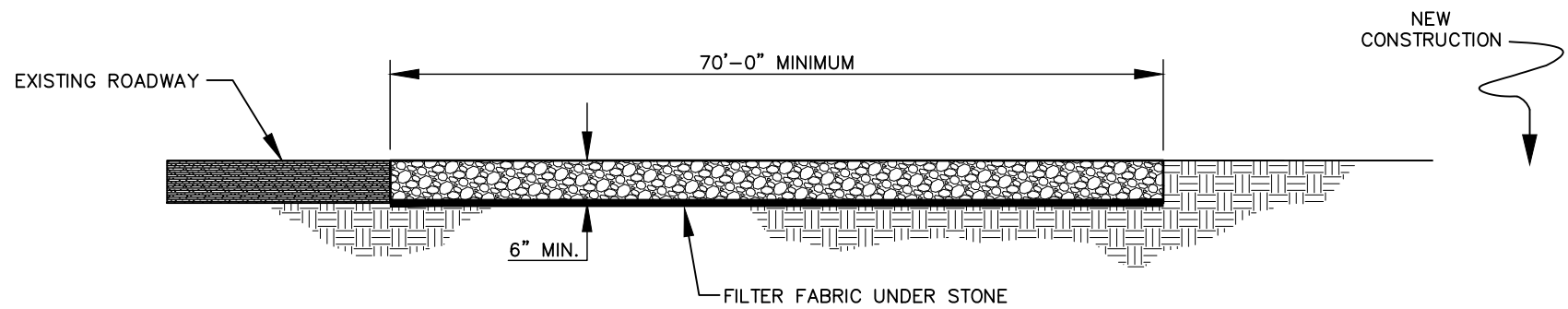
CROSS SECTION
