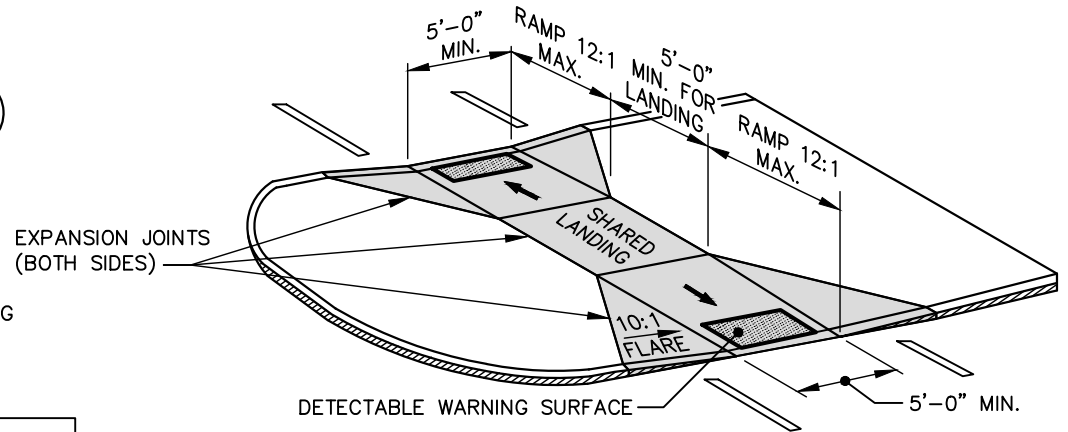
MEDIAN ISLAND CURB RAMPS
