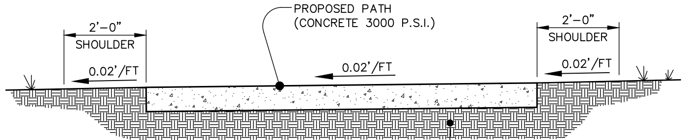
TYPICAL SECTION
