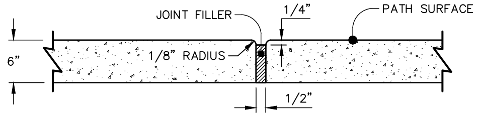
TRANSVERSE EXPANSION JOINT
