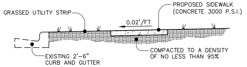
TYPICAL SECTION
