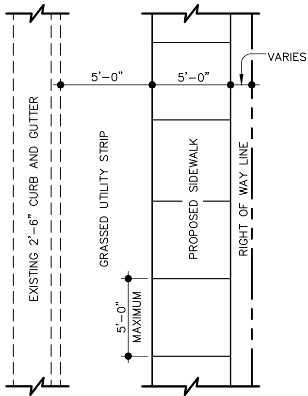
PLAN VIEW
